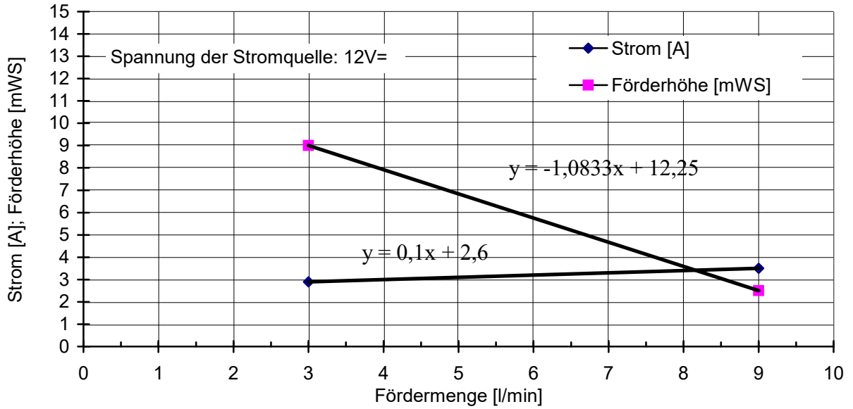
1900.57.00 Tauchpumpe COMET-COMBI 12-2T
