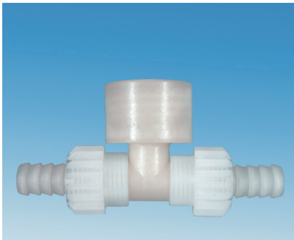
3191.00.01 T-connector on the pressure equalisation tank dimensions: 90 x 40 x 30 mm
